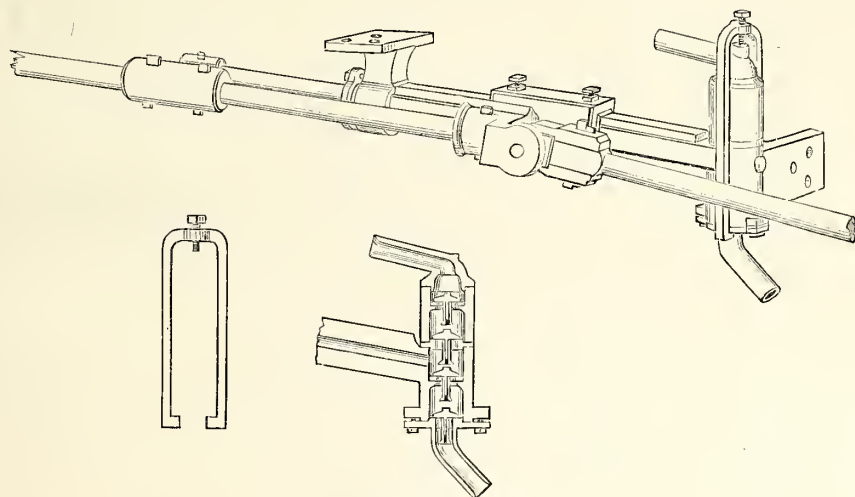
Fig. 5.—PUMP AND STIRRUP.
